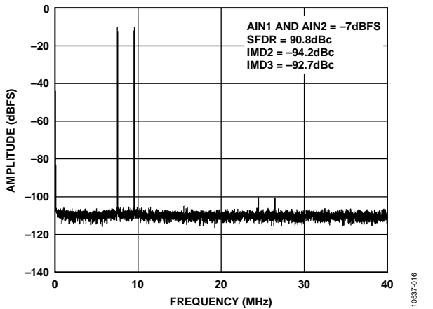
Figure 16. Two-Tone 16k FFT with f_{IN1} = 70.5 \text{ MHz} and f_{IN2} = 72.5 \text{ MHz} , f_{SAMPLE} = 80 \text{ MSPS}
